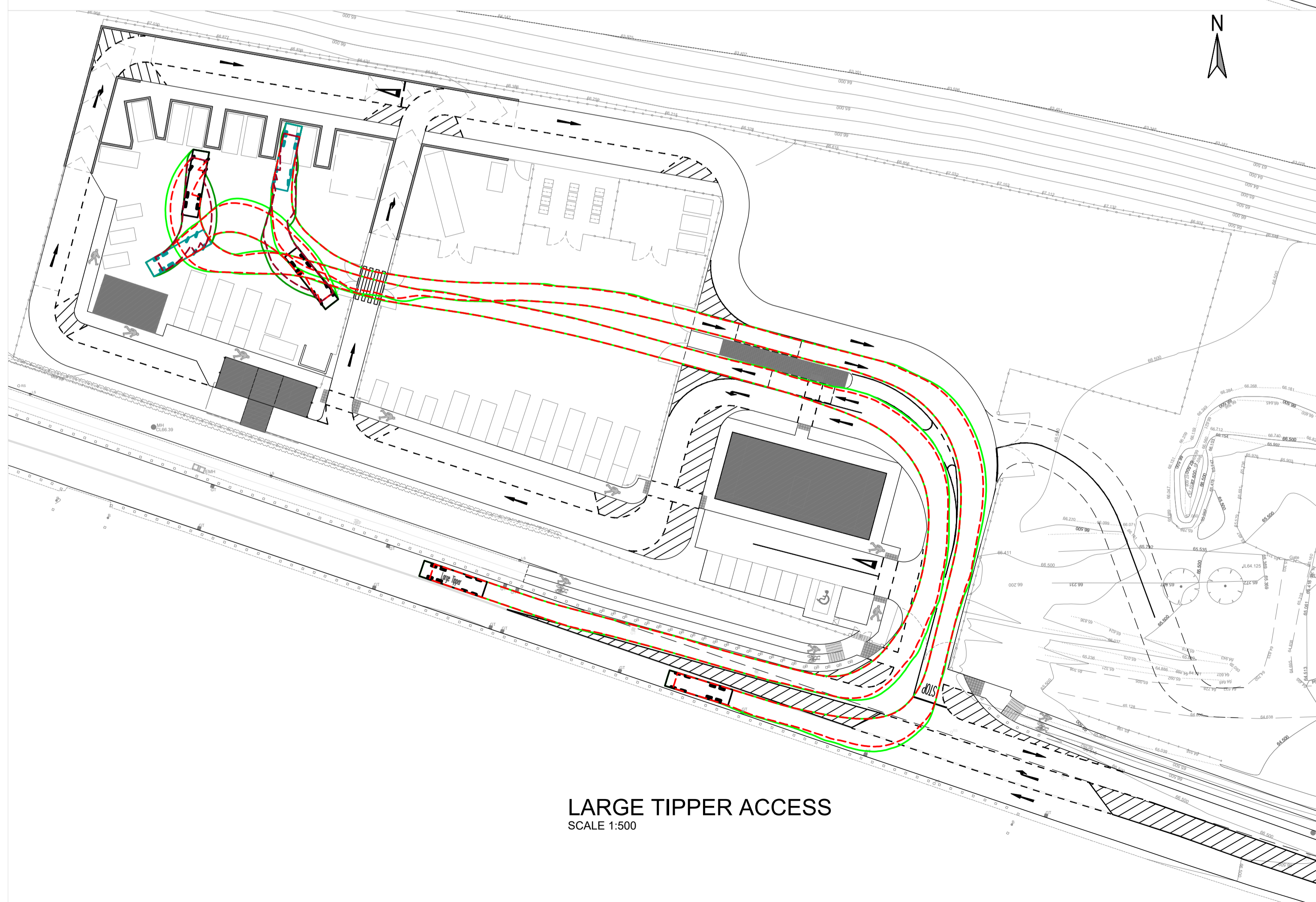
HGV ACCESS SCALE 1:500
