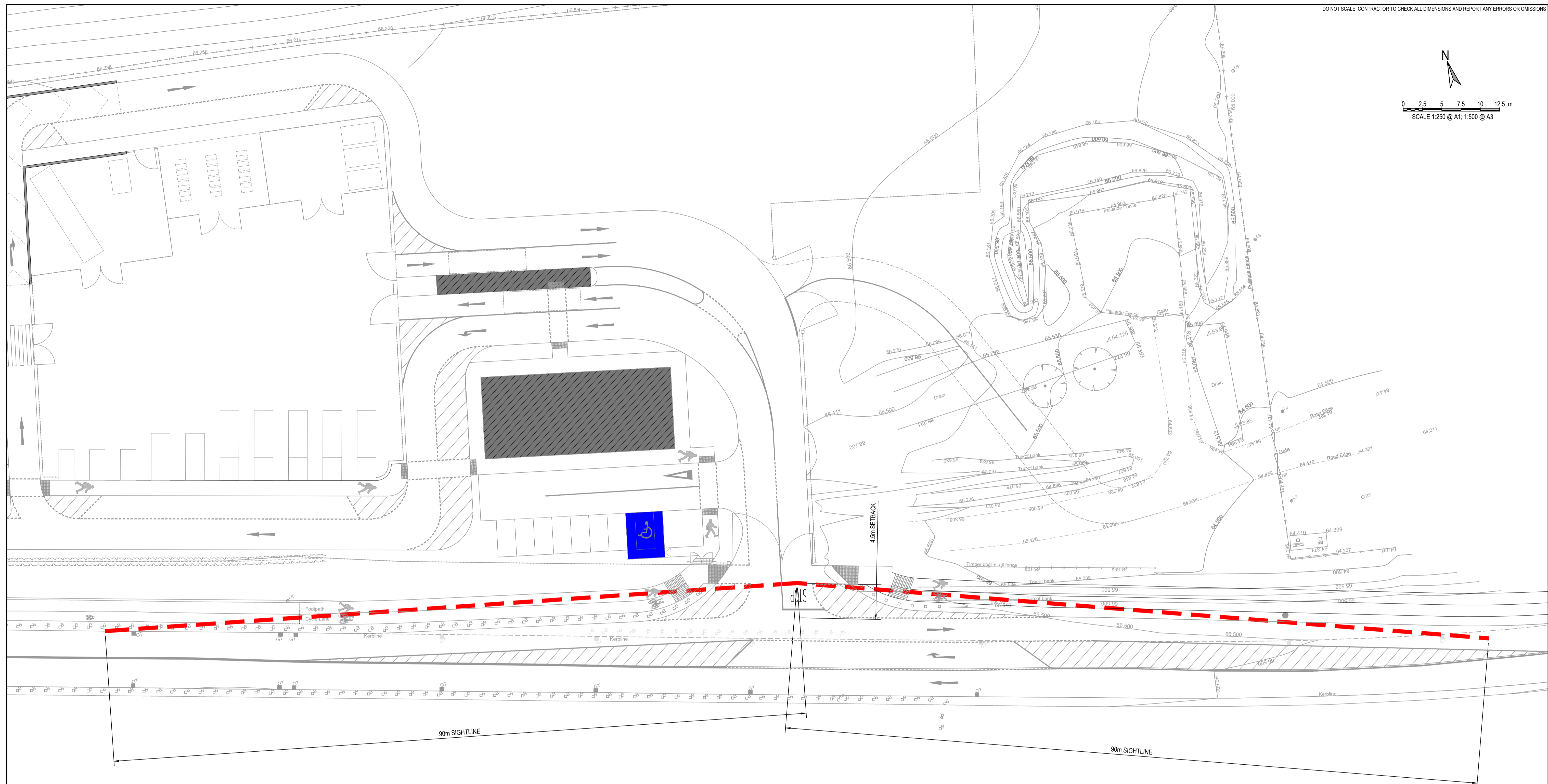
PROPOSED EXIT SIGHTLINES SCALE 1:250
