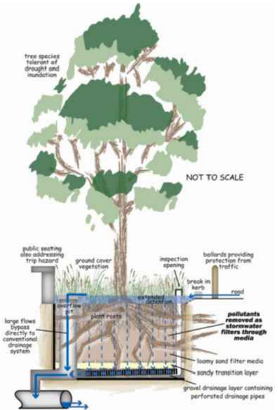
Typical Bio detention Tree Pit
