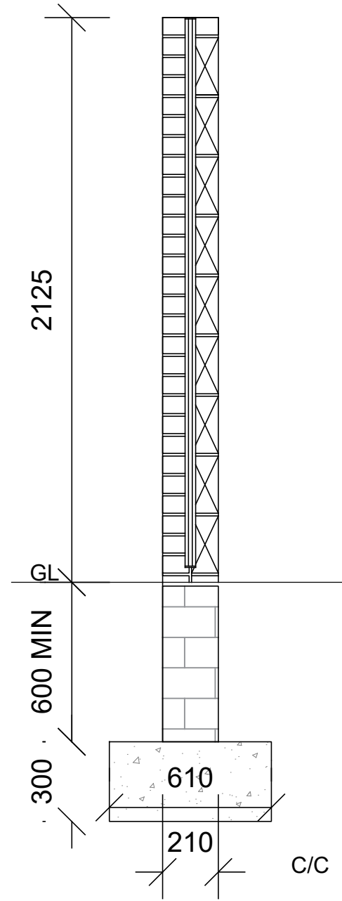
SECTION 1:20
