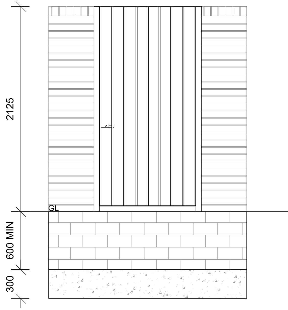
Typical Gate Elevation 1:20
