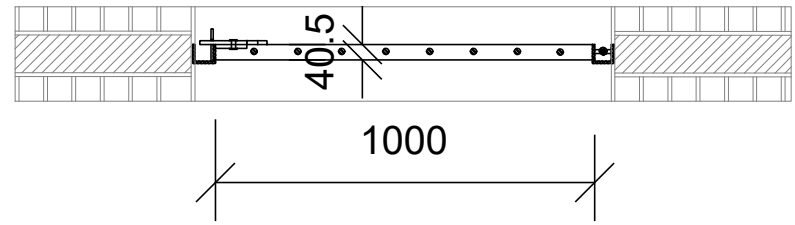
Typical Gate Plan 1:20
