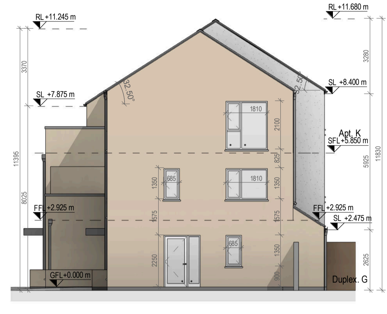
4 Side Elevation 2 1 : 100
