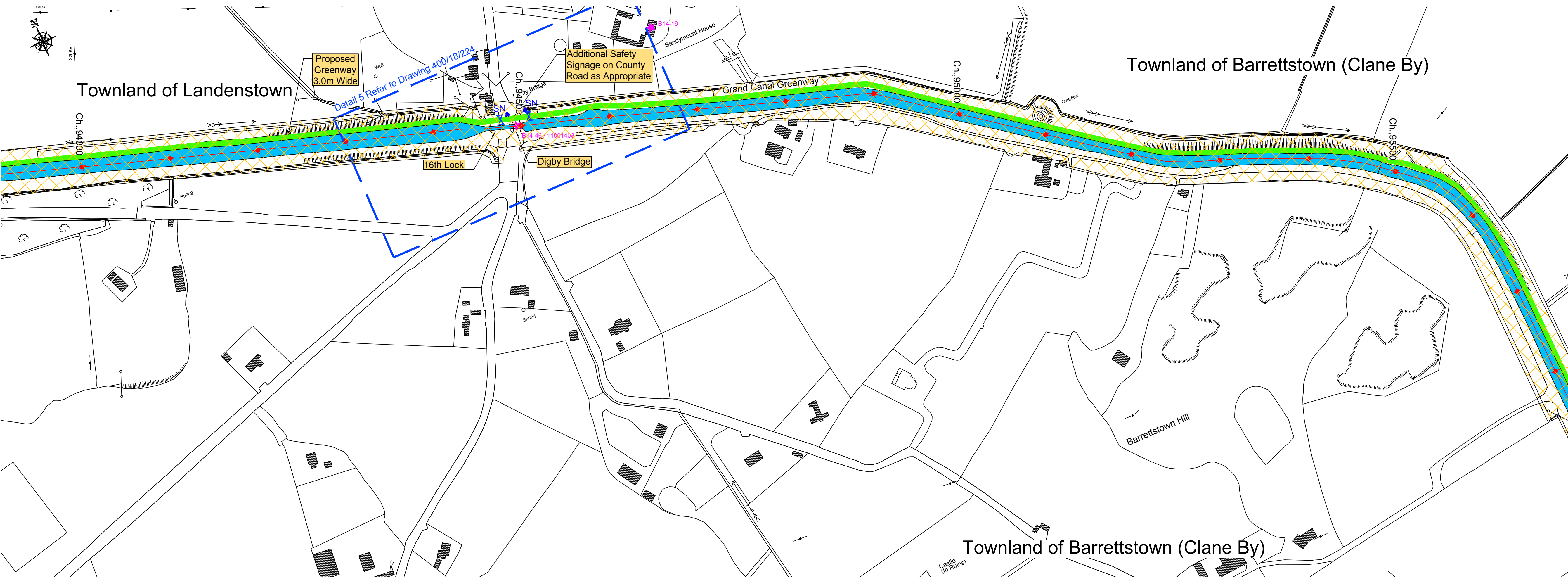
PLAN - SECTION K008 N
