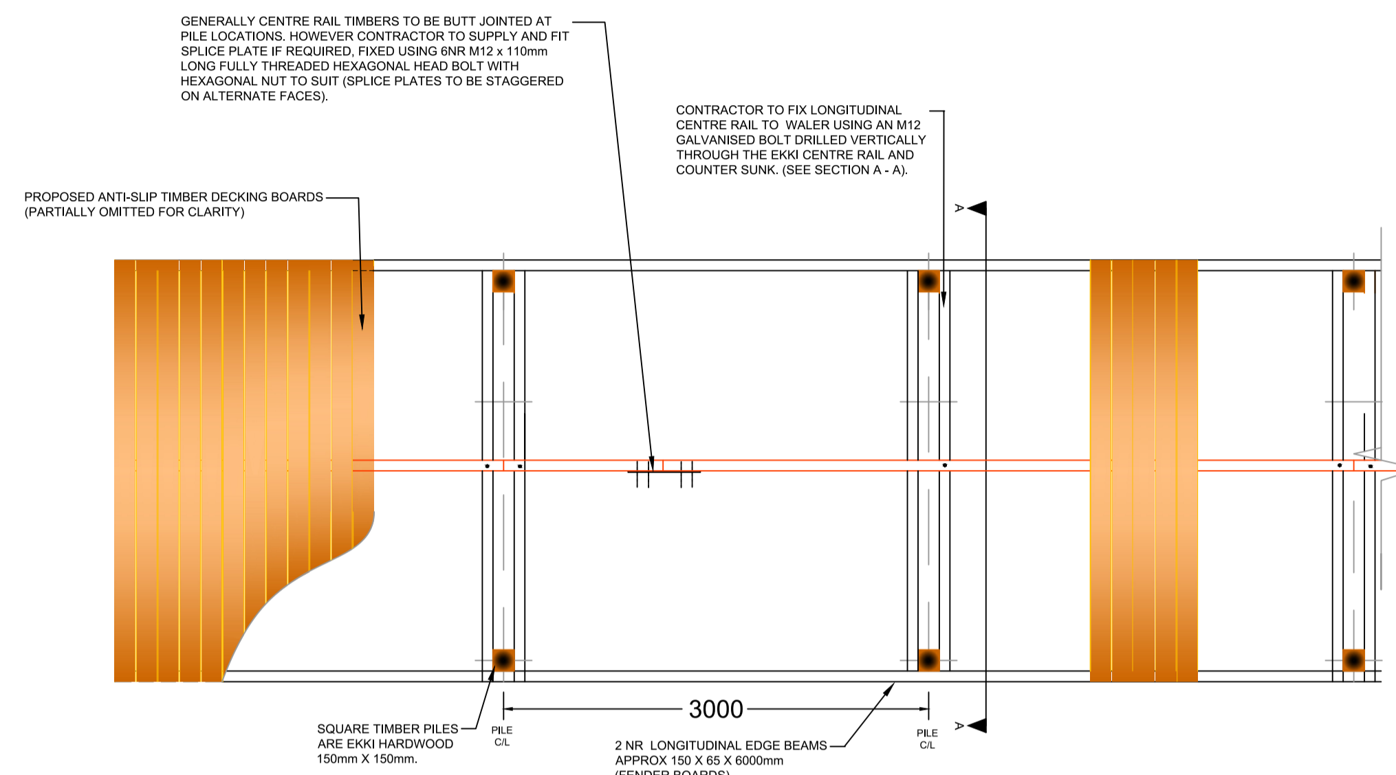
Typical Plan
