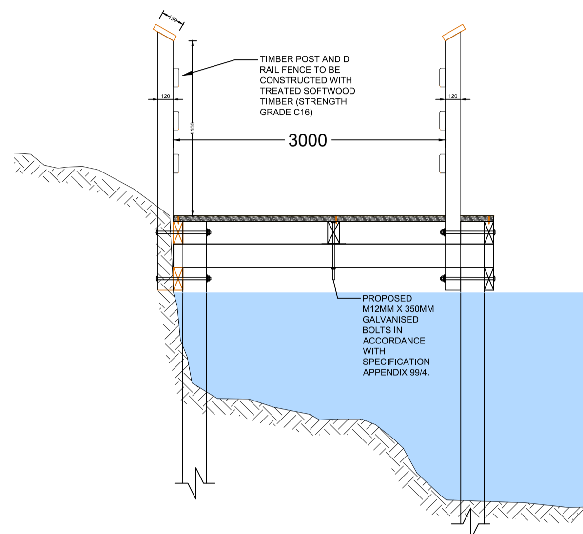
Typical Section
