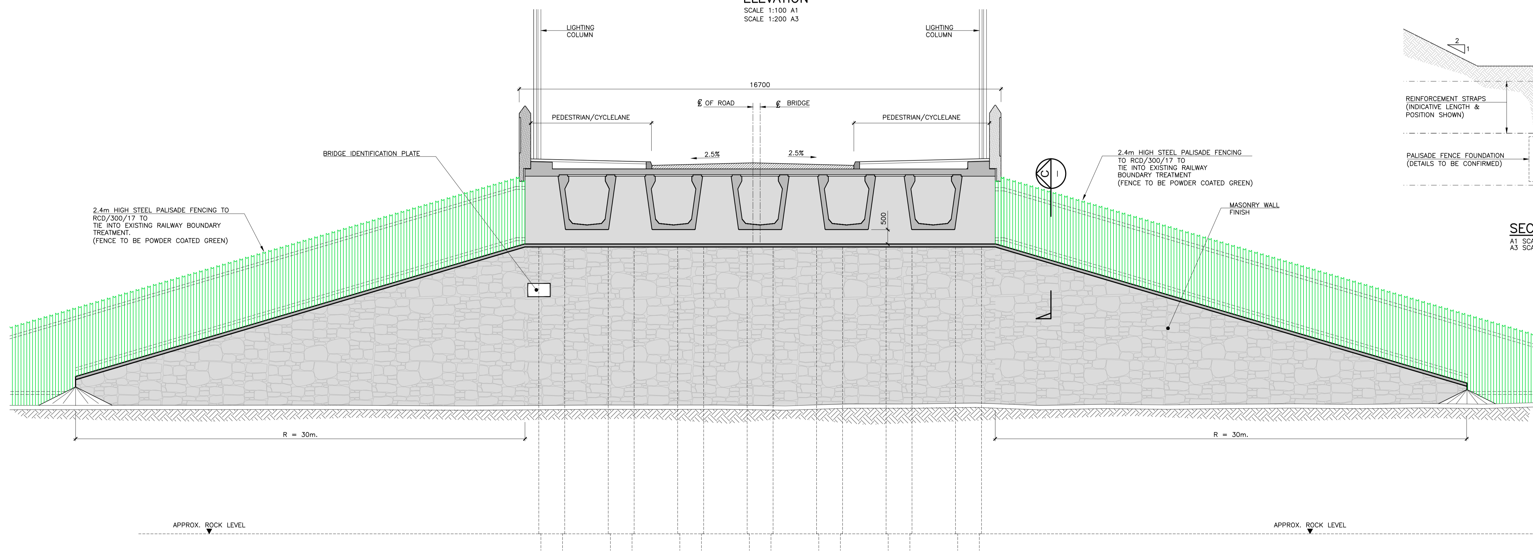
ELEVATION ON REINFORCED EARTH WALL SCALE 1:75 A1 SCALE 1:150 A3
