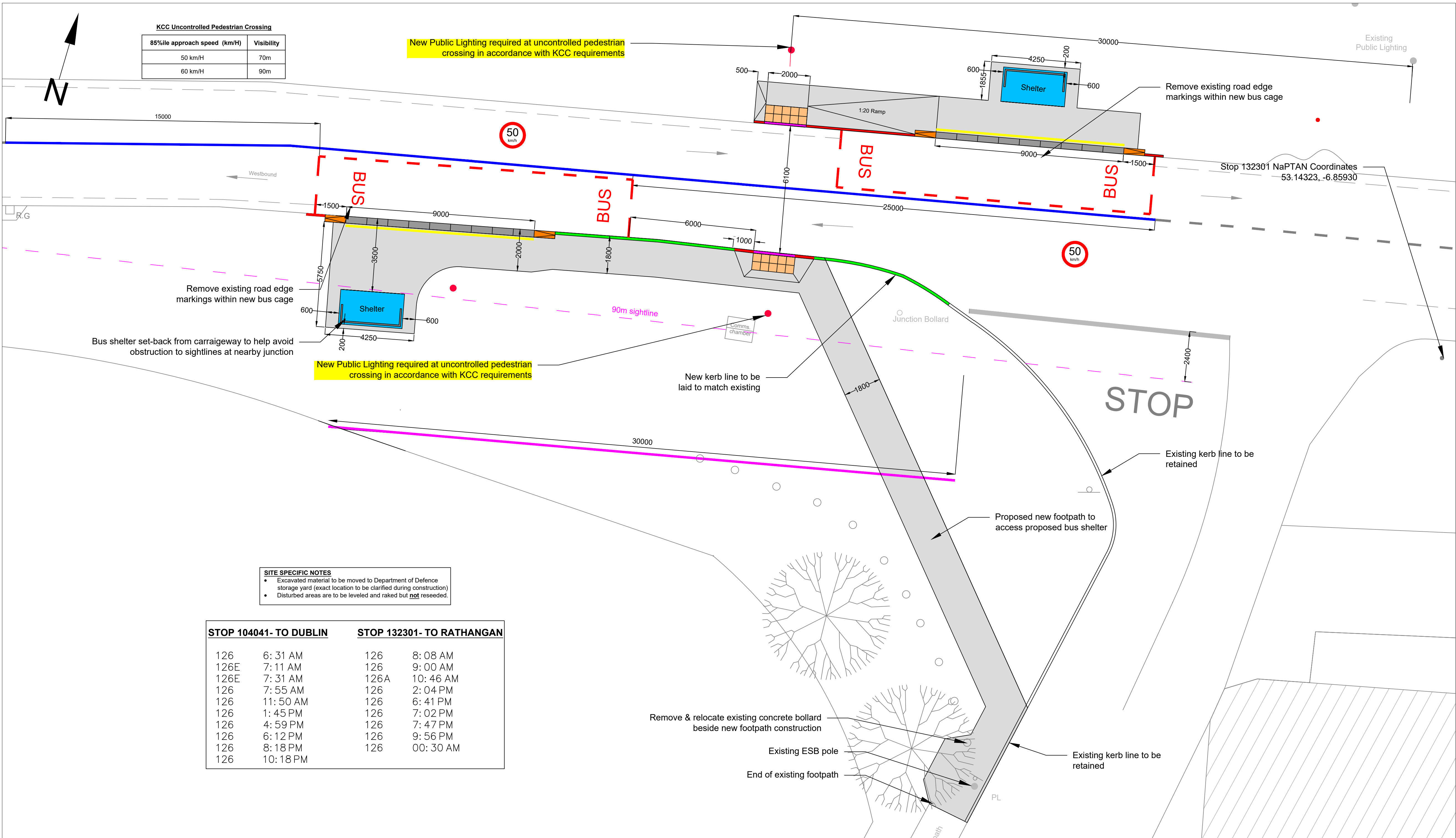
Figure 1 - Layout Plan Proposed new Bus Shelters/Boarding platforms
