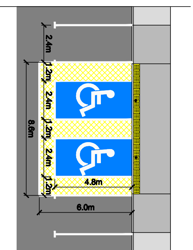
(Notes as option 2.) Multi Parking. Option 2.
