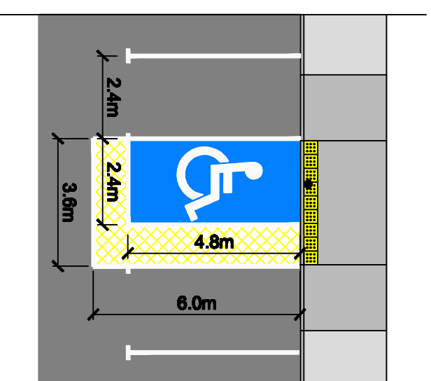
(Notes as option 1.) Perpendicular Parking. Option 2.
